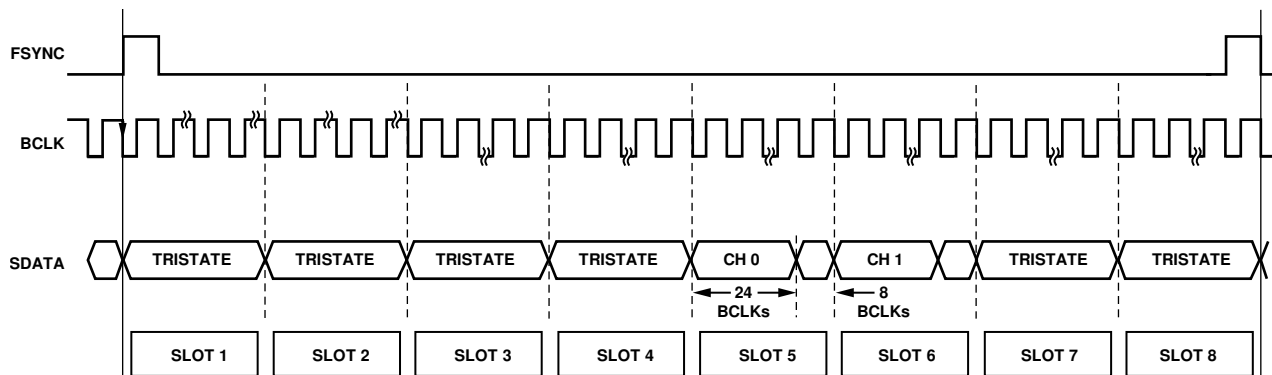
Figure 16. TDM-8, BCLK = 256 \times f_s , CONFIG Pin Tied to IOVDD Through a 47 kΩ Resistor
