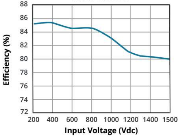
EFFICIENCY VS INPUT VOLTAGE AE40-UW-S24
