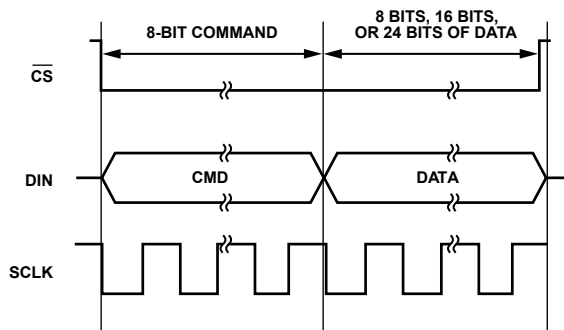
Figure 66. Writing to a Register (8-Bit Command with Register Address Followed by Data of 8 Bits, 16 Bits, or 24 Bits; Data Length Is Dependent on the Register Selected)
