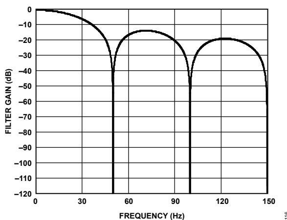
Figure 106. 50 Hz Rejection
