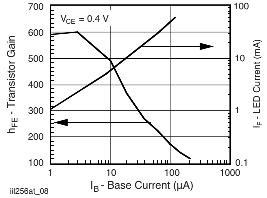
Fig. 8 - Base Current vs. I_F and h_{FE}
