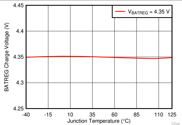
Figure 7-6. Battery Charge Voltage vs Junction Temperature
