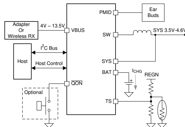
Simplified Application
