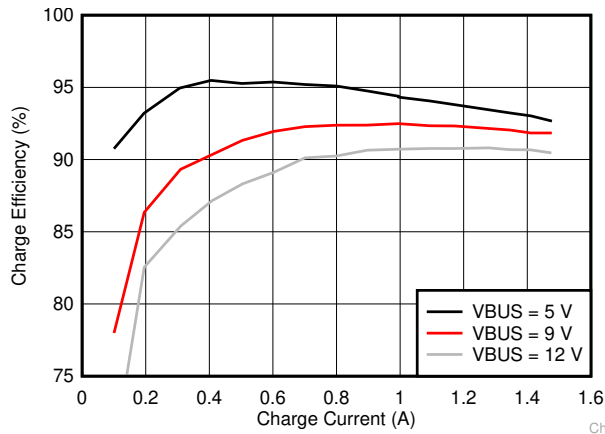
Figure 7-1. Charge Efficiency
