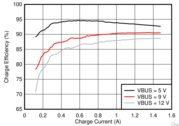
Figure 7-2. Charge Efficiency
