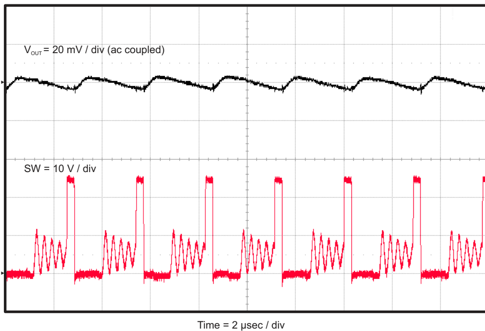
Figure 8. TPS54335EVM-556 Output Ripple, I_{OUT} = 100\text{ mA}
