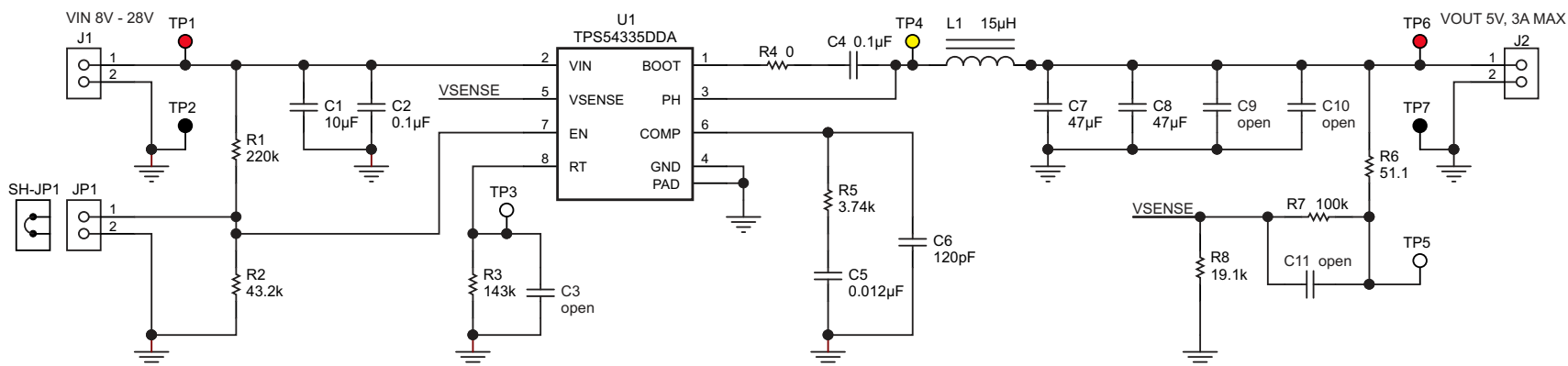
Figure 18. TPS54335EVM-556 Schematic
