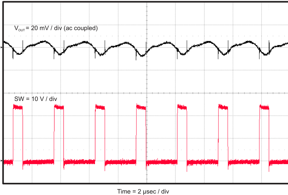
Figure 7. TPS54335EVM-556 Output Ripple, I_{OUT} = 3\text{ A}
