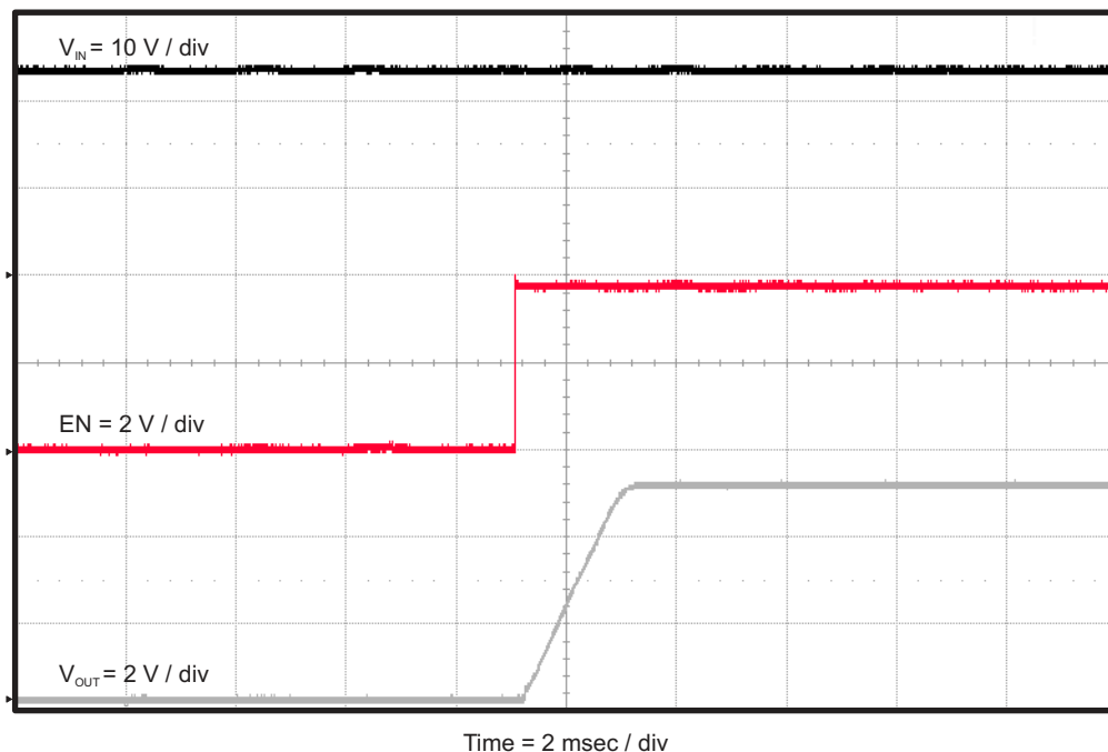
Figure 12. TPS54335EVM-556 Start-up Relative to Enable
