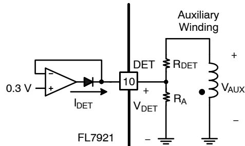
Figure 38. Valley Detection
