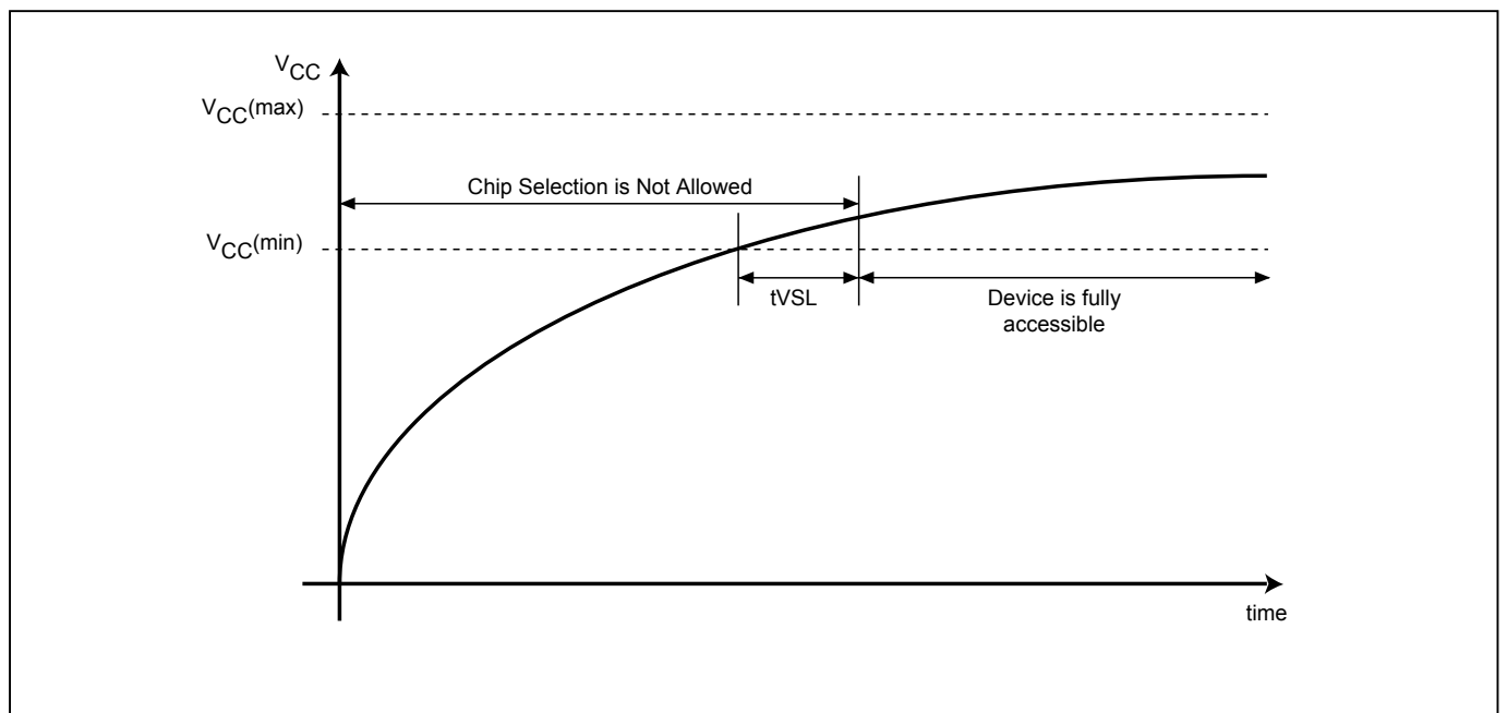
Figure 34. Power-up Timing
