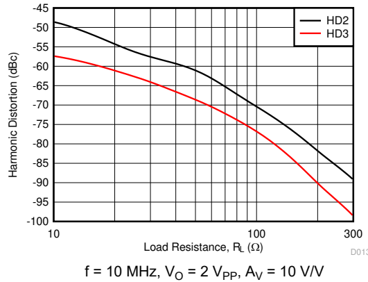
Figure 6-22. Harmonic Distortion vs R_L
