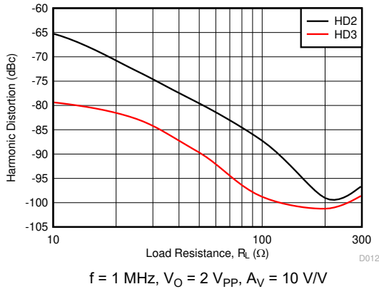
Figure 6-21. Harmonic Distortion vs R_L
