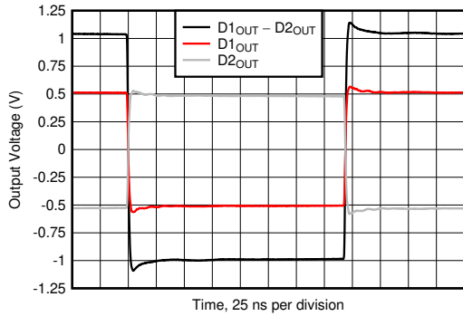
Figure 6-49. Small-Signal Pulse Response
