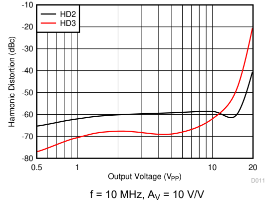
Figure 6-20. Harmonic Distortion vs V_O
