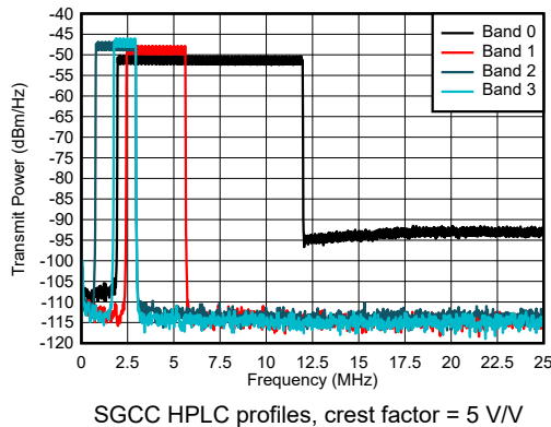
Figure 6-3. Out-of-Band Suppression
