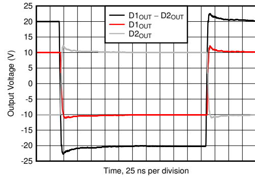
Figure 6-50. Large-Signal Pulse Response
