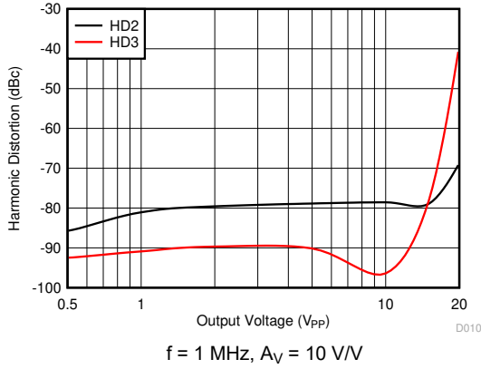
Figure 6-19. Harmonic Distortion vs V_O
