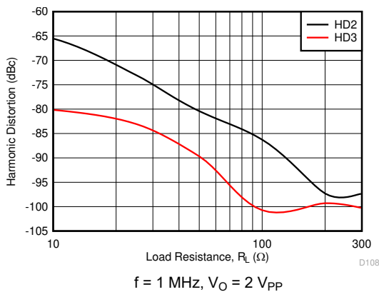
Figure 6-47. Harmonic Distortion vs R_L
