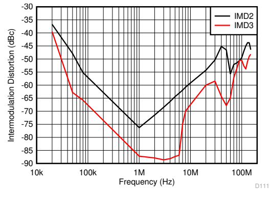
Figure 6-42. Intermodulation Distortion vs Frequency
