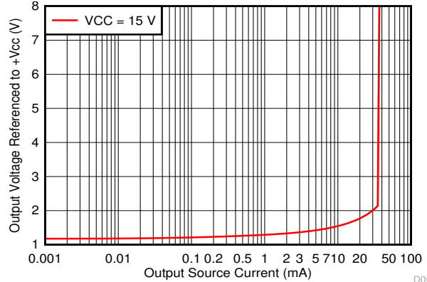
Figure 6-36. Output Sourcing Characteristics
