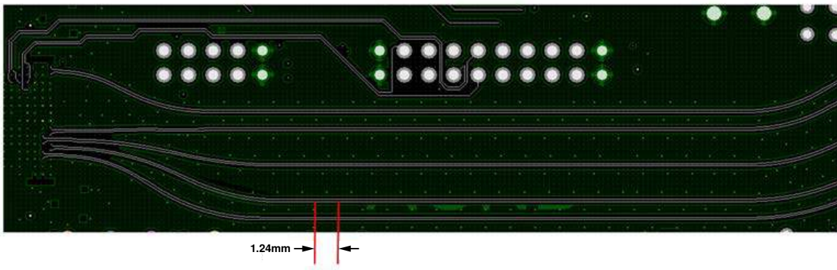
Figure 182. Via Fencing Around JESD204B Lines, PCB Layer 10
