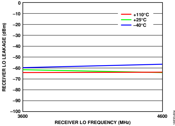
Figure 102. Receiver LO Leakage from 3600 MHz to 4600 MHz, 0 dB Attenuation, 200 MHz RF Bandwidth, 245.76 MSPS Sample Rate
