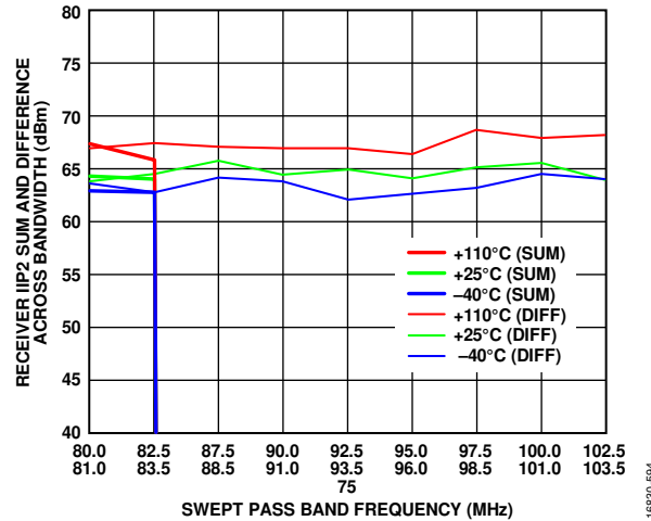
Figure 16. Receiver IIP2 Sum and Difference Across Bandwidth vs. Swept Pass Band Frequency, Receiver Attenuation = 0 dB, LO = 75 MHz, 10 Tone Pairs, -23.5 dBm Each
