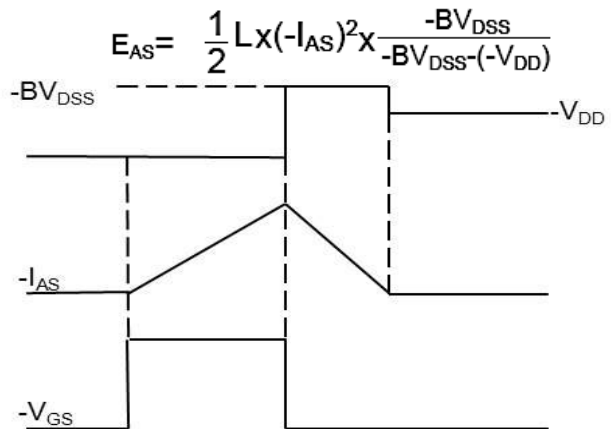
Figure 10. EAS Waveform
