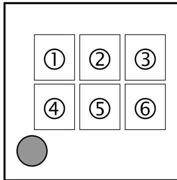
R5524K (DFN(PL)1820-6) Part Markings
