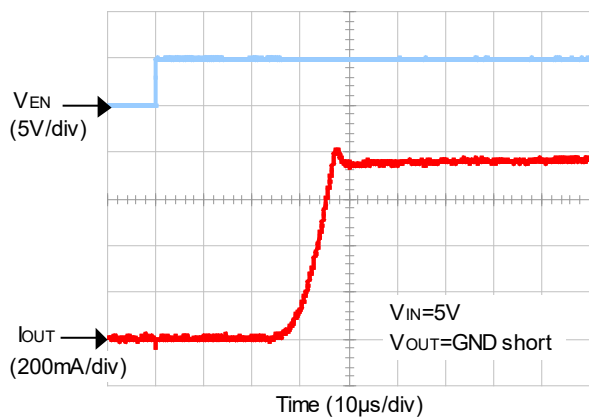
22) Overcurrent Limit Transient Response (Output short during enable "H")
