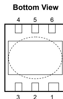
R5524K (DFN(PL)1820-6) Pin Configuration
