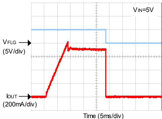
21) Overcurrent Response with Ramped Load (R5524x004A)
