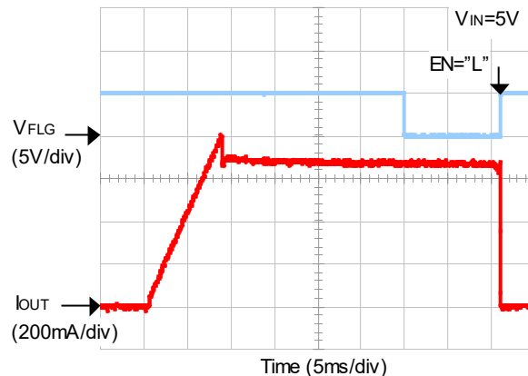
20) Overcurrent Response with Ramped Load (R5524x002x)
