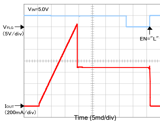
21) Overcurrent Response with Ramped Load (R5524x004A)
