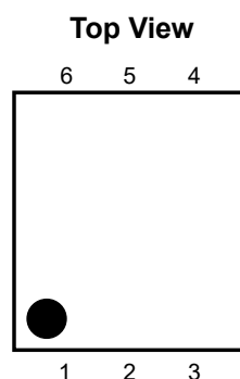
R5524K (DFN(PL)1820-6) Pin Configuration
