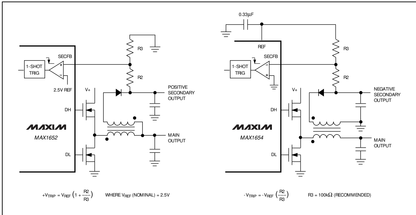
Figure 7. Secondary-Output Feedback Dividers
