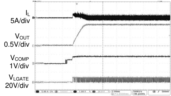
Time 2ms/div
