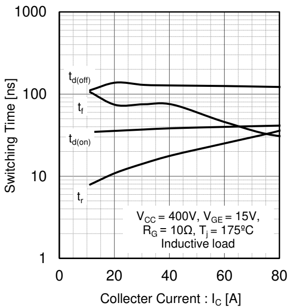
Fig.11 Typical Switching Time vs. Collector Current
