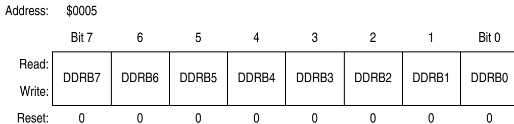
Figure 20-6. Data Direction Register B (DDRB)
