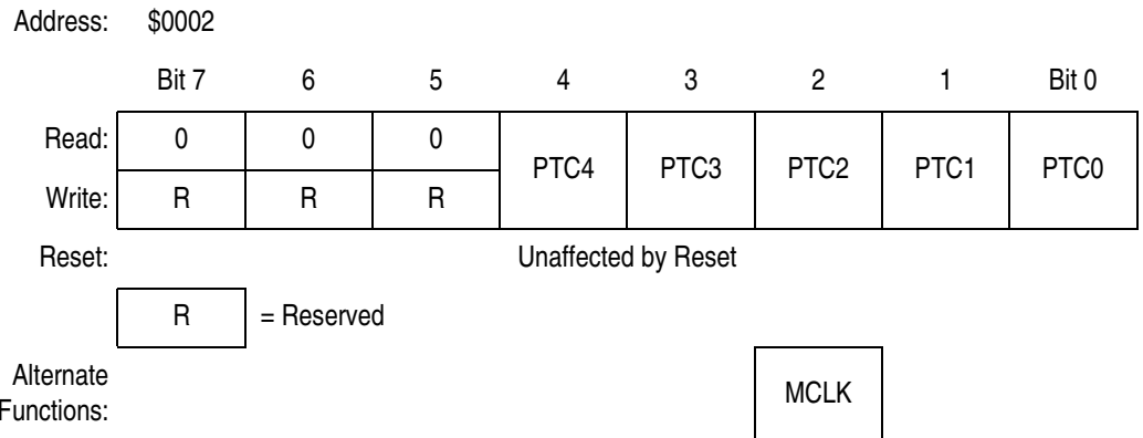
Figure 20-8. Port C Data Register (PTC)
