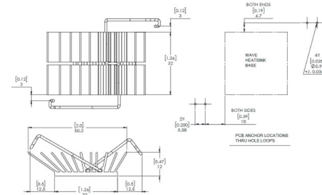
MECHANICAL DIMENSIONS
