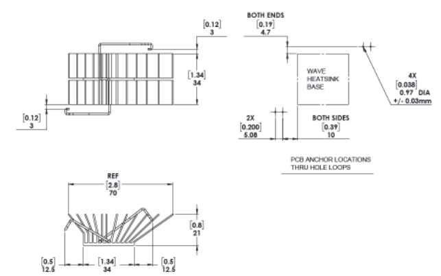
MECHANICAL DIMENSIONS
