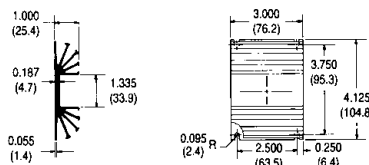
641 SERIES (EXTRUSION PROFILE 1371)
