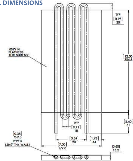
MECHANICAL DIMENSIONS
