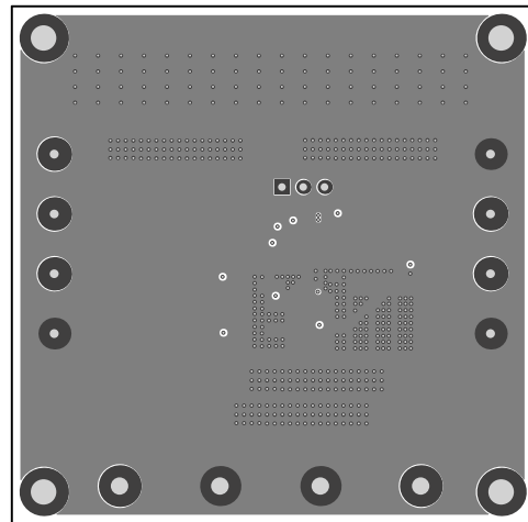
Figure 4—Inner Layer 2
