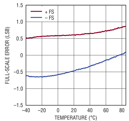
Full-Scale Error vs Temperature, \text{REFBUF} = 4.096\text{V}
