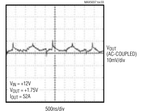
OUTPUT RIPPLE
