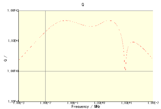
CLF10040T-680M-CA
