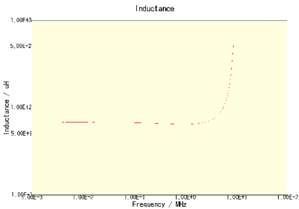
CLF10040T-680M-CA
