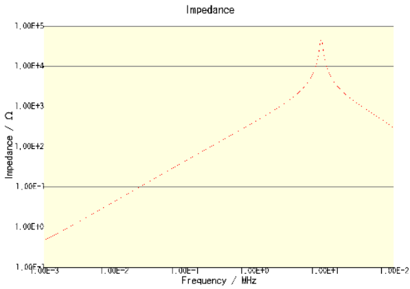
CLF10040T-680M-CA
