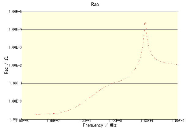
CLF10040T-680M-CA
