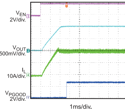
Power Up through EN I_{OUT} = 20A
