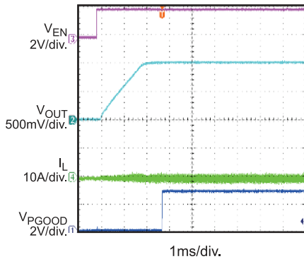
Power Up through EN I_{OUT} = 0A
