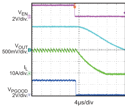
Power Down through EN I_{OUT} = 20A
