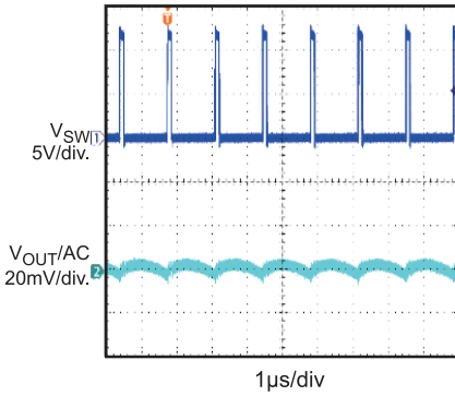
Steady State I_{OUT} = 0A
