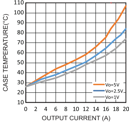
Thermal Results
