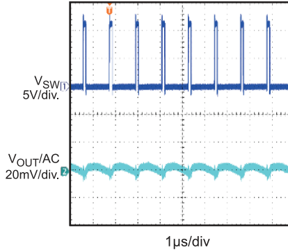
Steady State I_{OUT} = 20A
