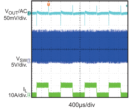
Load Transient I_{OUT} = 0A \sim 8A
