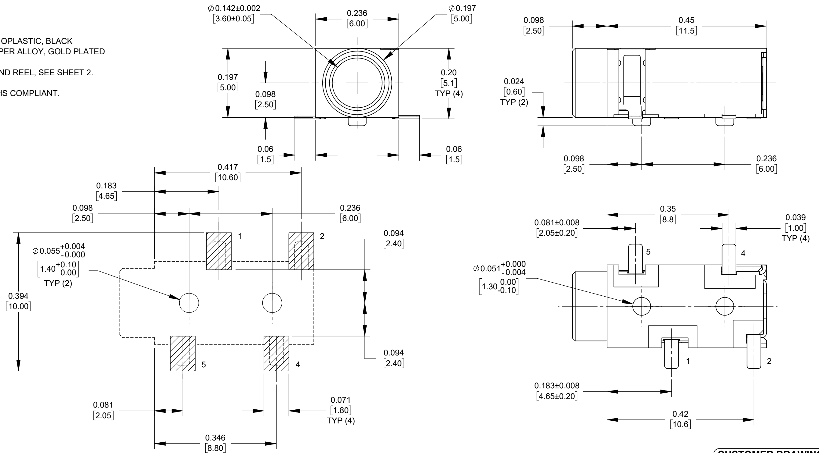
PCB LAYOUT COMPONENT SIDE
