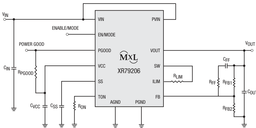
Figure 1. Typical Application
