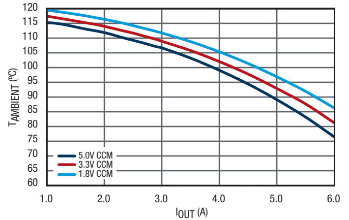
Figure 21. Maximum T_{\text{AMBIENT}} vs. I_{\text{OUT}} , V_{IN} = 12\text{V}
