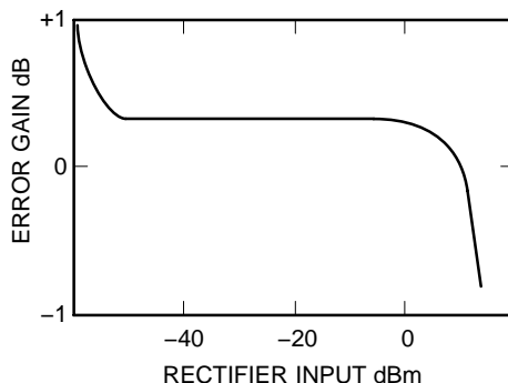
Figure 10. Rectifier Accuracy
