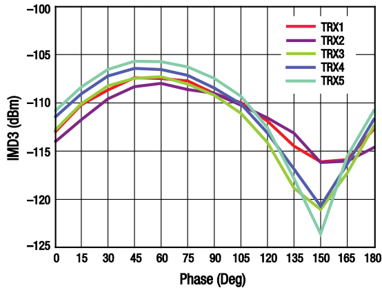
Figure 17. 3 rd Order Intermodulation Distortion vs Phase, TRX Ports ( f_{FUND} = 1.95 GHz, f_{BLK} = 1.76 GHz, f_{RX} = 2.14 GHz)
