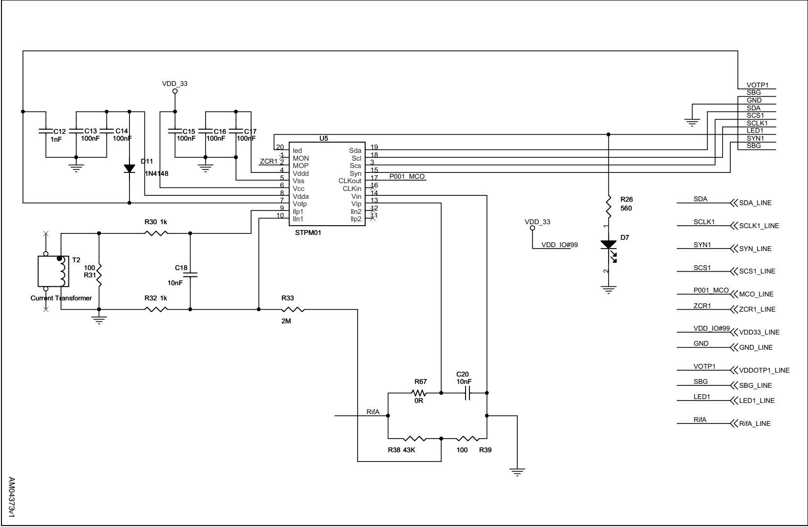
Figure 6. Differential current meter
