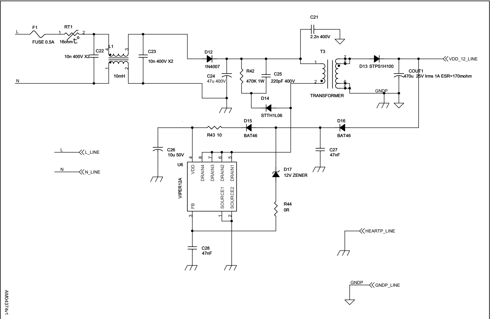
Figure 7. AC/DC converter
