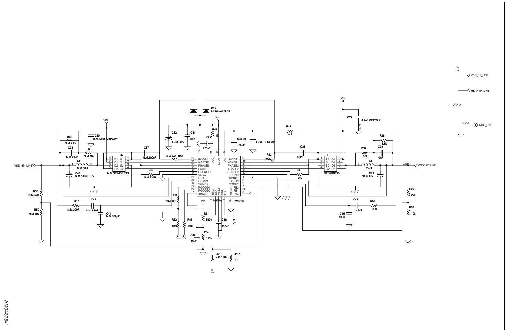
Figure 8. DC/DC converter
