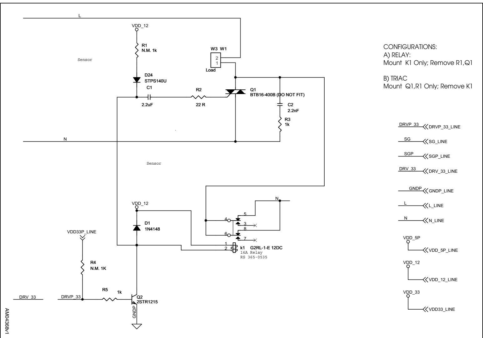
Figure 1. AC load driver page
