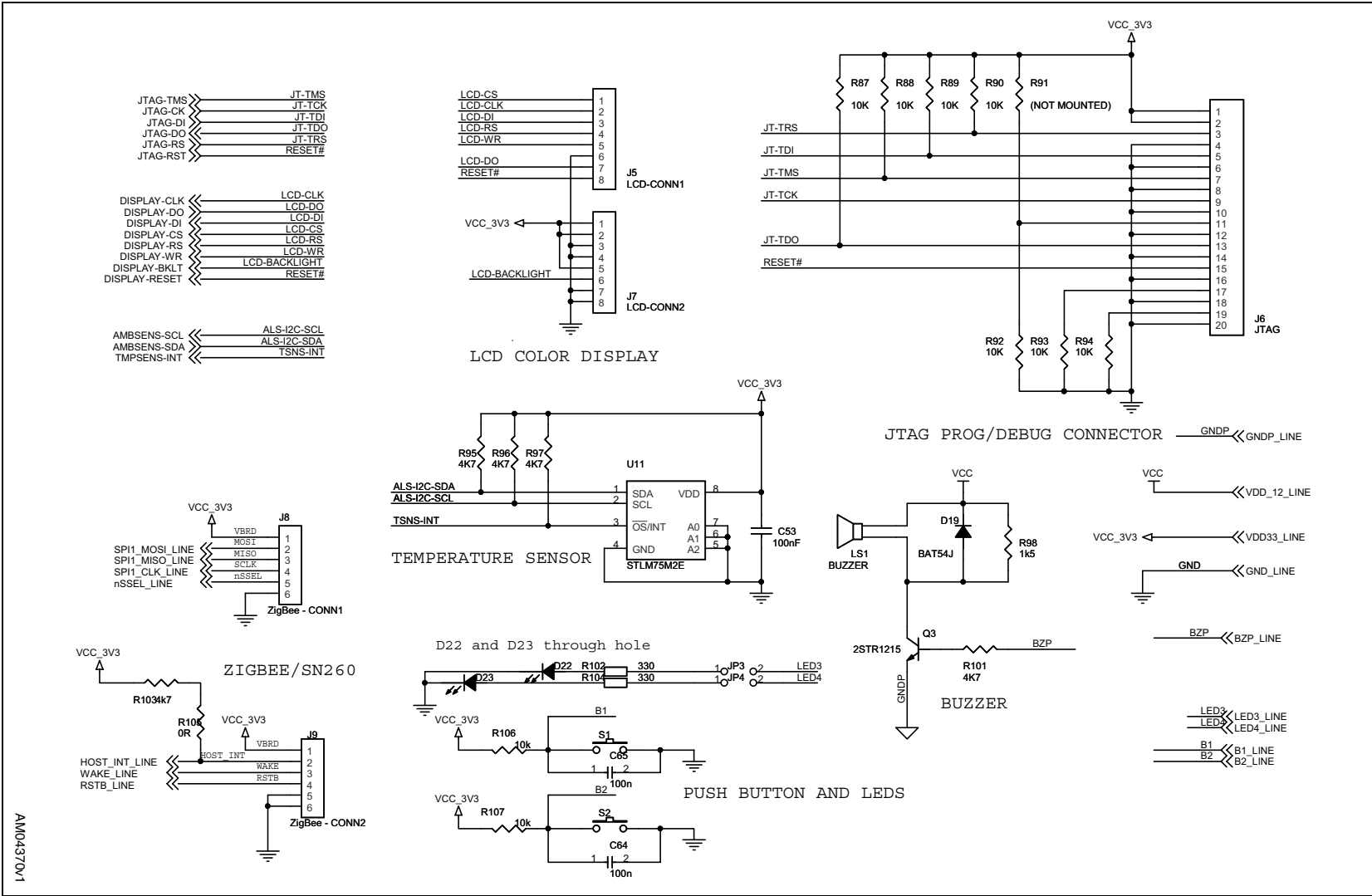
Figure 3. Temperature sensor and connectors
