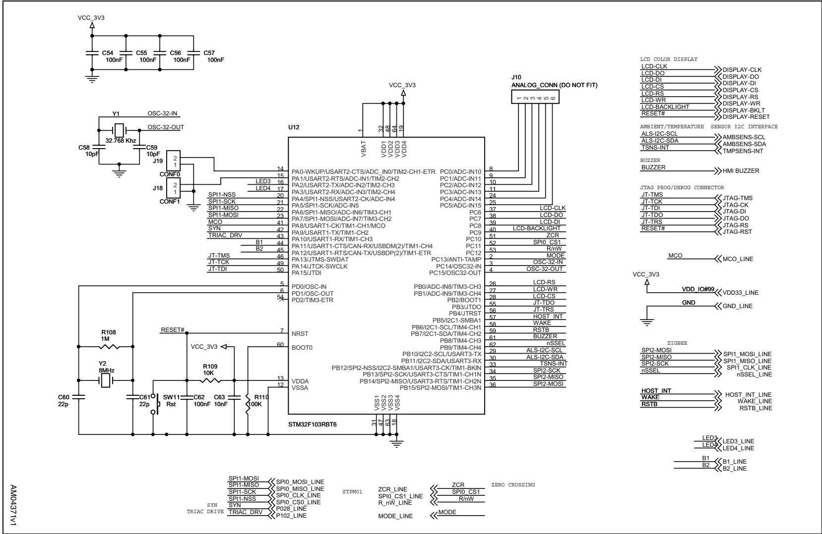
Figure 4. Microcontroller
