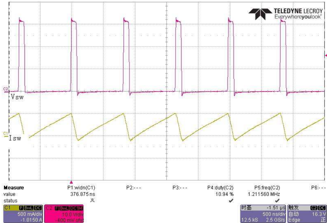
Vsw&Isw Waveform(VCC=3.6V Iout=20mA 10 WLED String)
