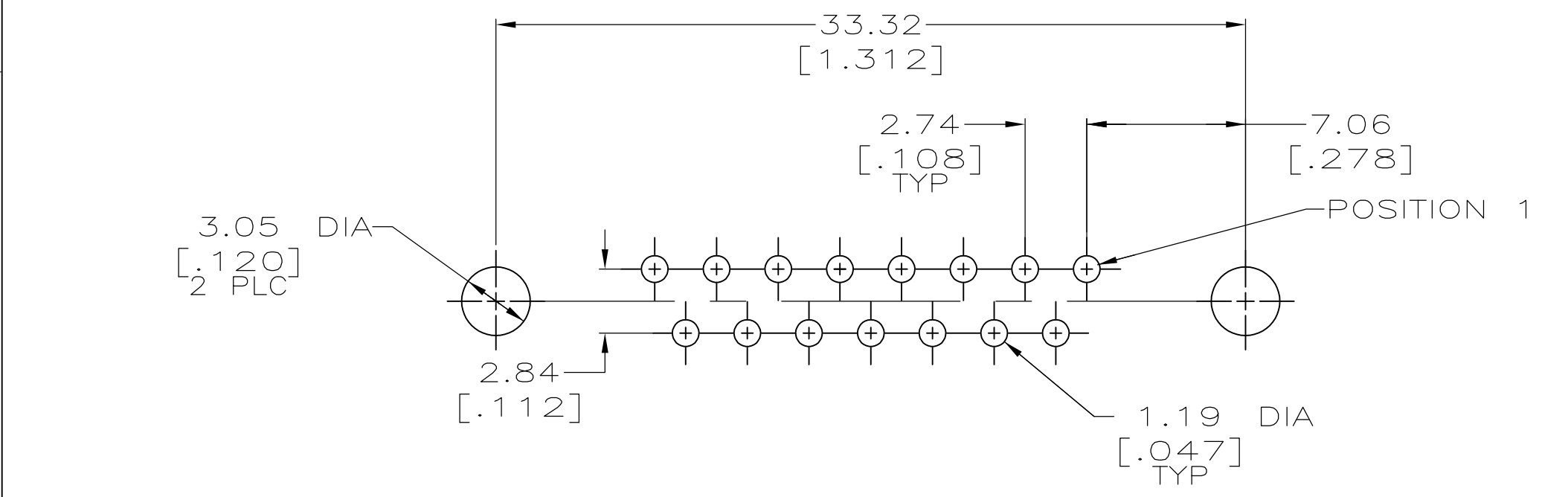
P.C. BOARD MOUNTING DIMENSIONS
