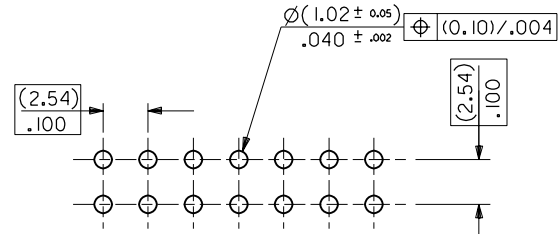
RECOMMENDED P.C. BOARD HOLE PATTERN 2 B 1 B SH. REV.
