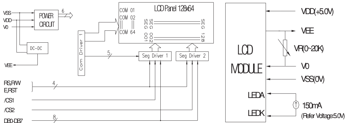
Figure 1. Block Diagram
