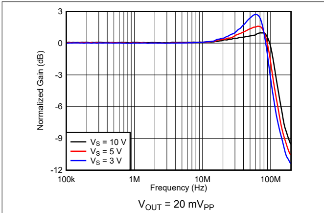
Figure 7-43. Frequency Response vs Supply Voltage
