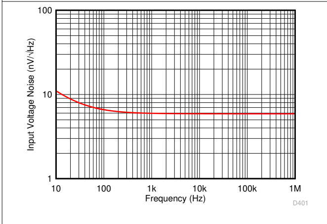
Figure 7-45. Input Voltage Noise Density vs Frequency
