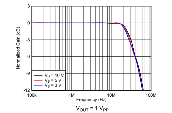
Figure 7-44. Frequency Response vs Supply Voltage
