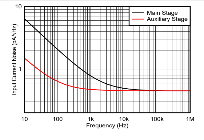
Figure 7-46. Input Current Noise Density vs Frequency
