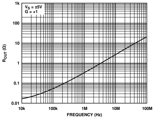
Figure 48. AD9632 Output Resistance vs. Frequency
