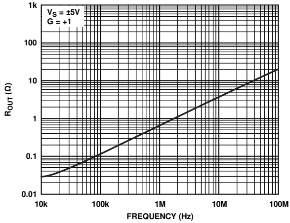
Figure 47. AD9631 Output Resistance vs. Frequency
