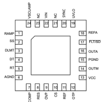
QFN24 (Top View)
