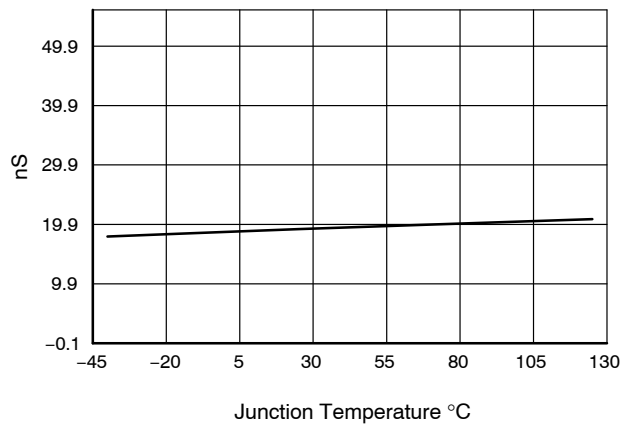
t_{LIMSC}(DELAY)
