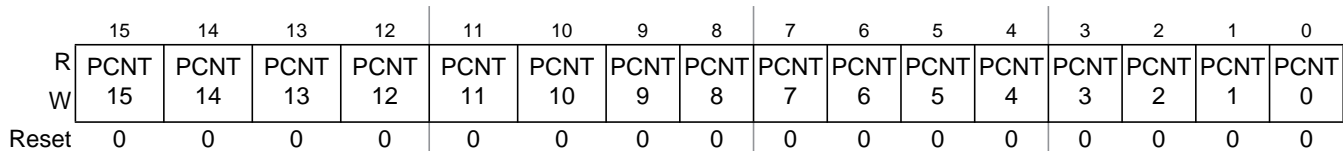
Figure 13-18. PIT Count Register 3 (PITCNT3)
