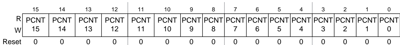
Figure 13-17. PIT Count Register 2 (PITCNT2)
