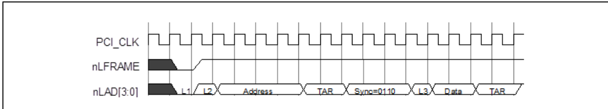
FIGURE 22-8: I/O READ
