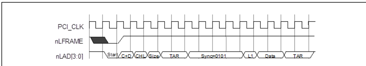
FIGURE 22-10: DMA WRITE (FIRST BYTE)
