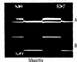
MAX752 LOAD TRANSIENT RESPONSE
