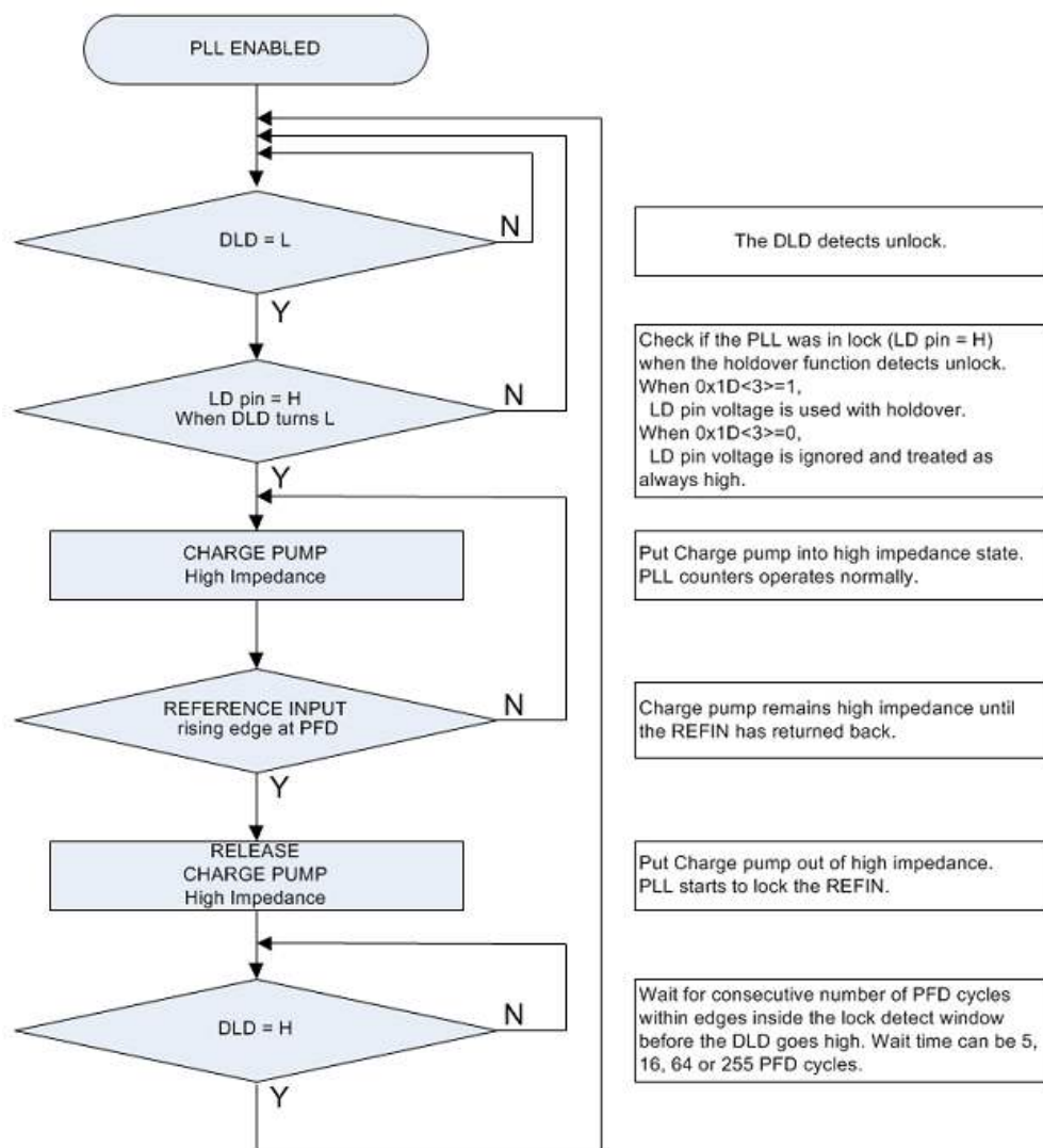
Figure 19. Automatic Holdover
