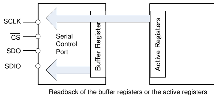
Figure 32. Readback Registers
