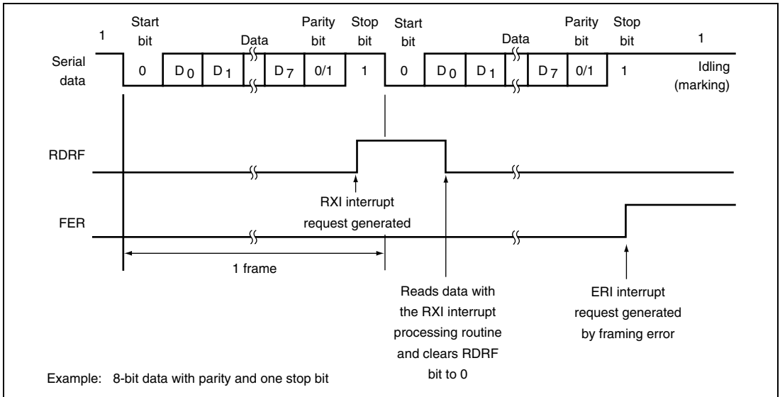
Figure 14.11 SCI Receive Operation
