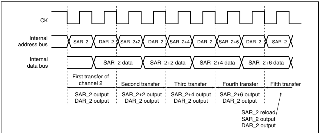
Figure 9.25 Timing Chart of Source Address Reload Function
