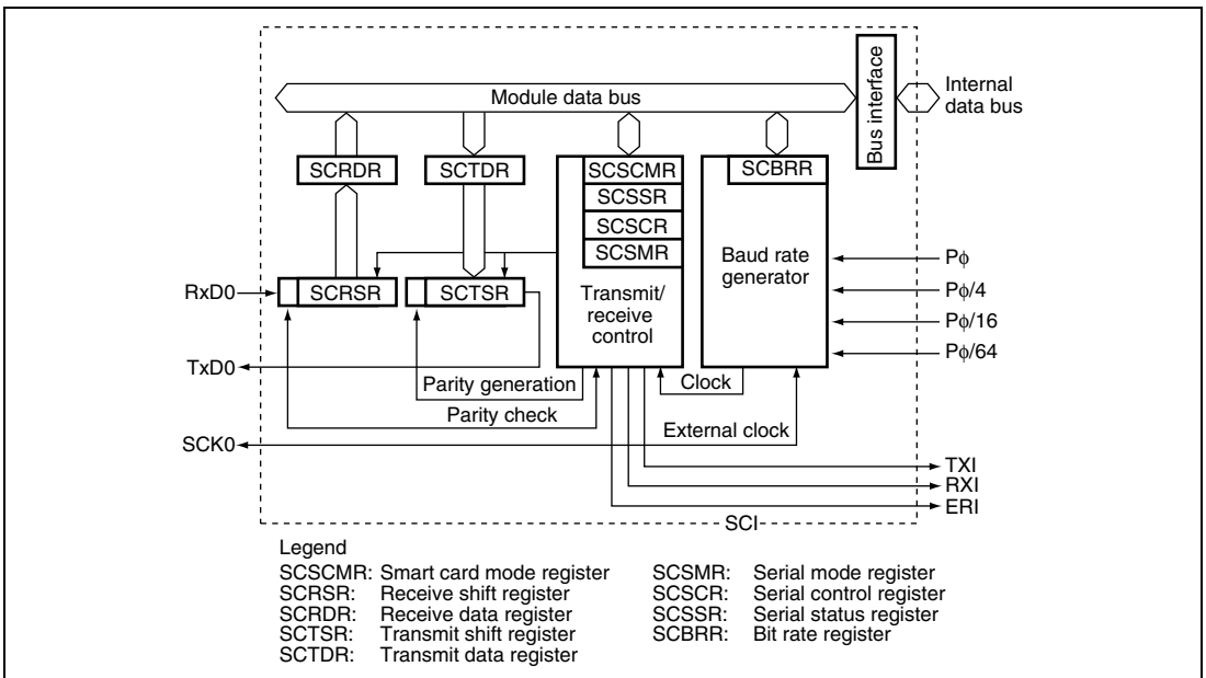
Figure 15.1 Smart Card Interface Block Diagram
