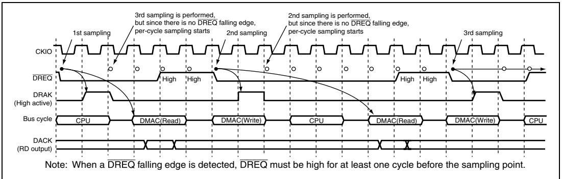
Figure 9.21 Cycle-Steal Mode, Edge input (CPU Access: 2 Cycles)
