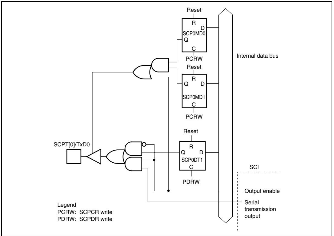
Figure 14.3 SCPT[0]/TxD0 Pin
