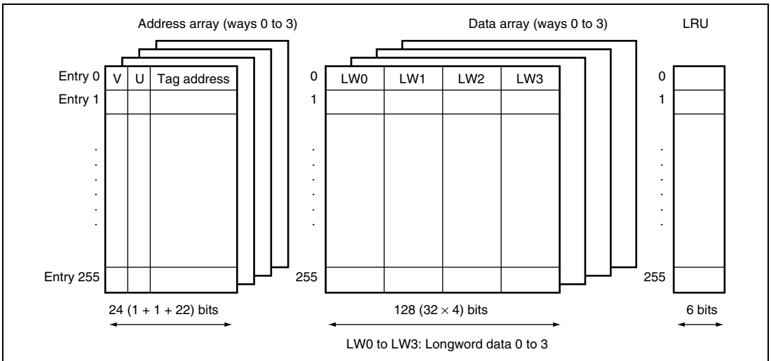
Figure 5.1 Cache Structure
