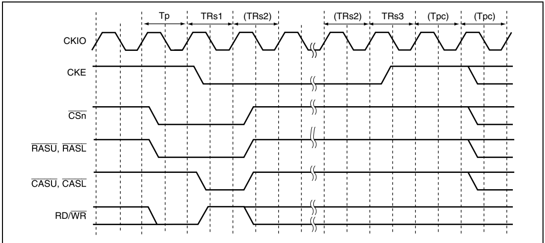
Figure 8.26 Synchronous DRAM Self-Refresh Timing
