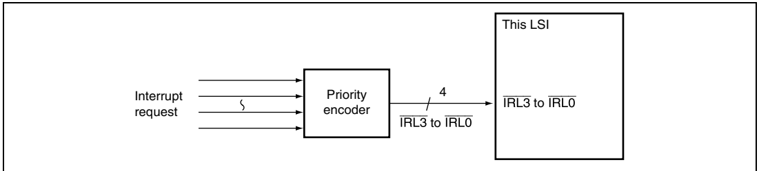
Figure 6.2 Example of IRL Interrupt Connection
