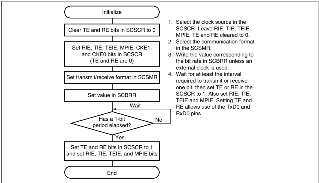
Figure 14.18 Sample Flowchart for SCI Initialization
