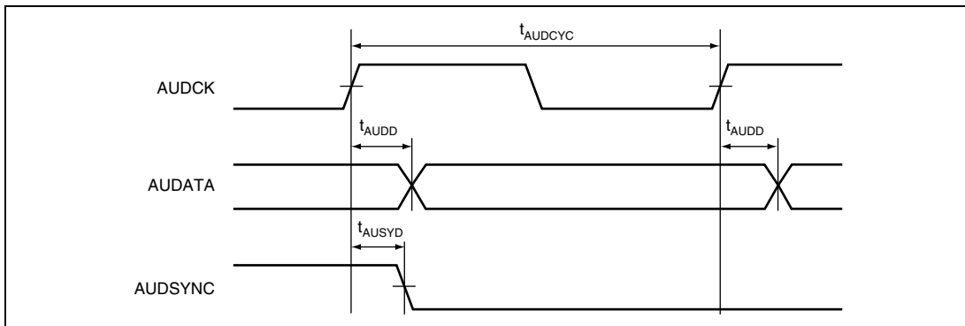
Figure 24.59 AUD Timing
