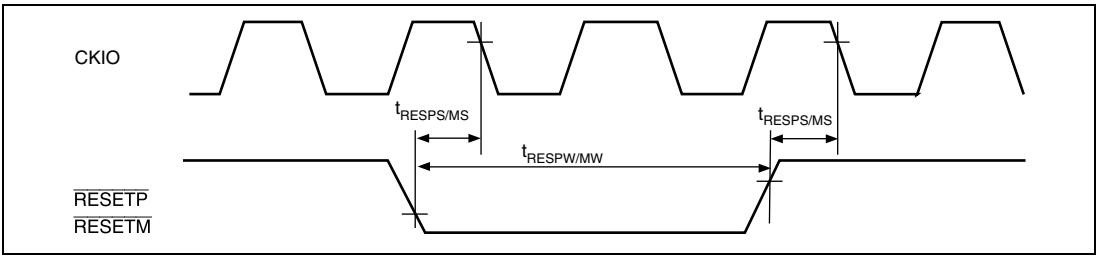
Figure 24.11 Reset Input Timing
