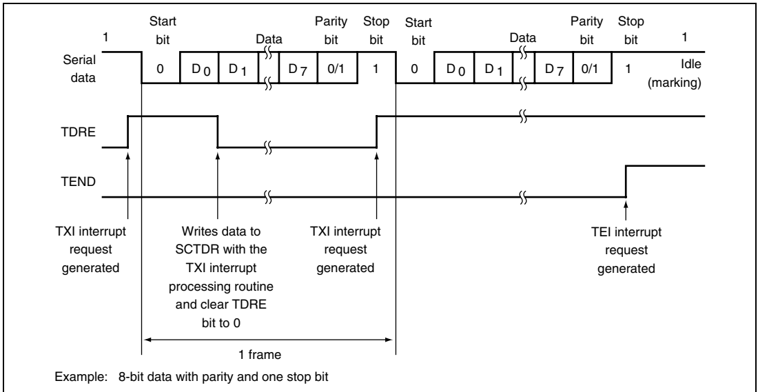
Figure 14.9 SCI Transmit Operation in Asynchronous Mode
