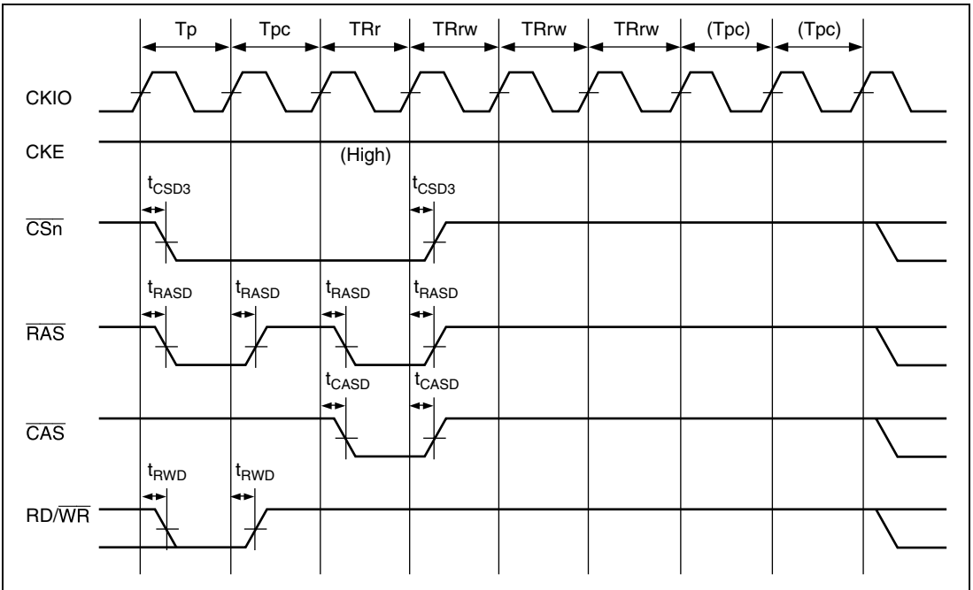
Figure 24.37 Synchronous DRAM Auto-Refresh Timing ( TRAS = 1 , TPC = 1 )
