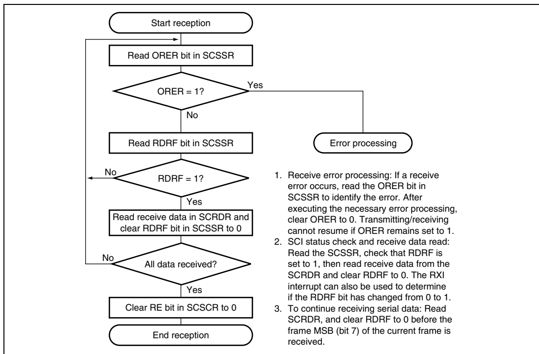
Figure 14.21 Sample Flowchart for Serial Data Receiving
