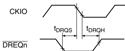
Figure 24.53 \overline{DREQ} Input Timing
