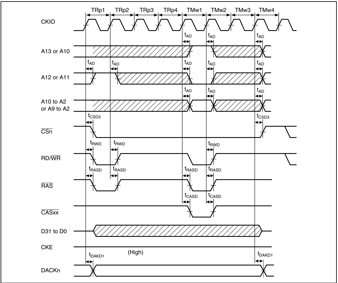
Figure 24.39 Synchronous DRAM Mode Register Write Cycle
