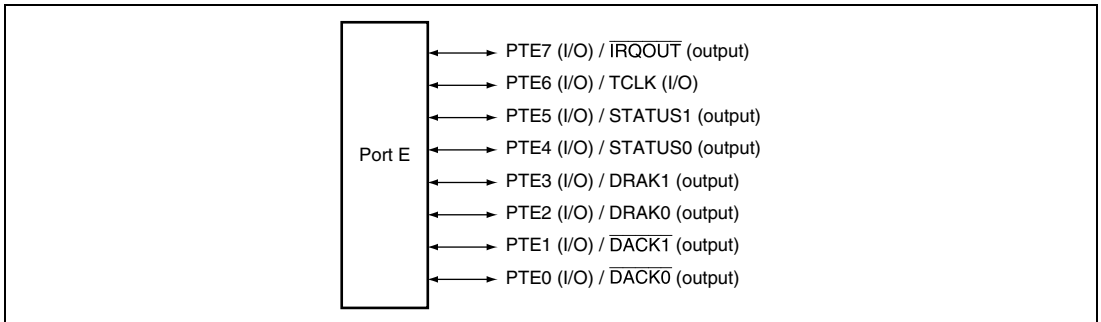
Figure 18.5 Port E
