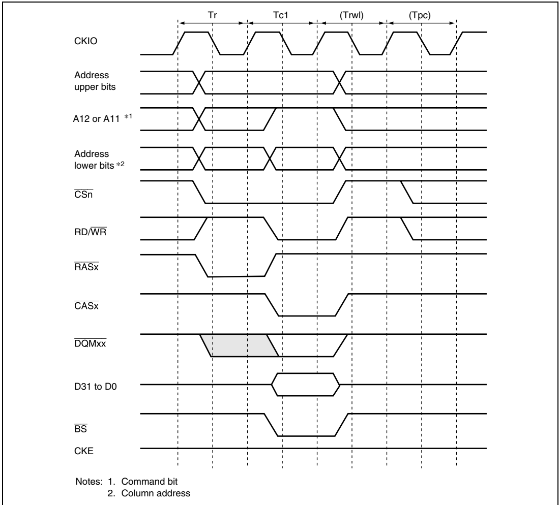
Figure 8.17 Basic Timing for Synchronous DRAM Single Write
