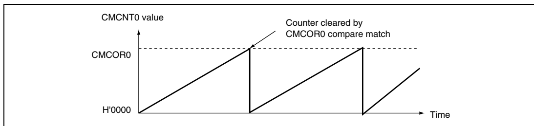
Figure 9.27 Counter Operation
