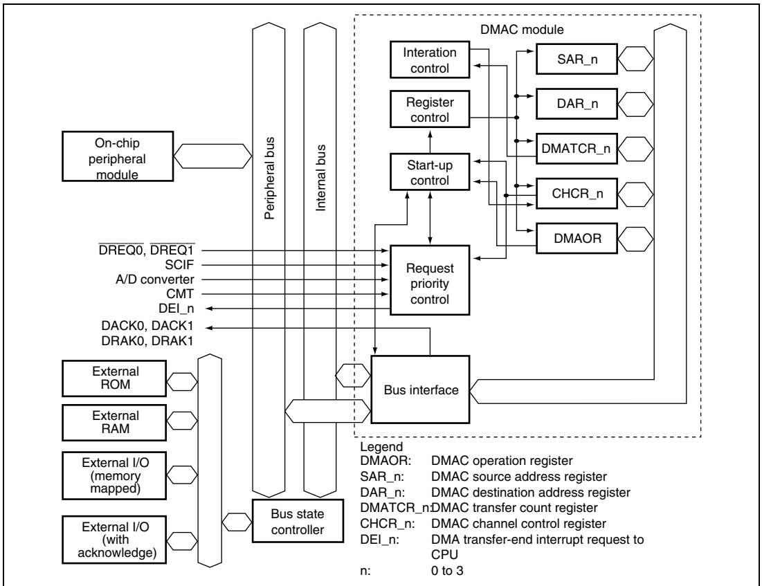
Figure 9.1 DMAC Block Diagram
