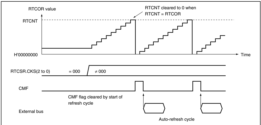
Figure 8.24 Auto-Refresh Operation
