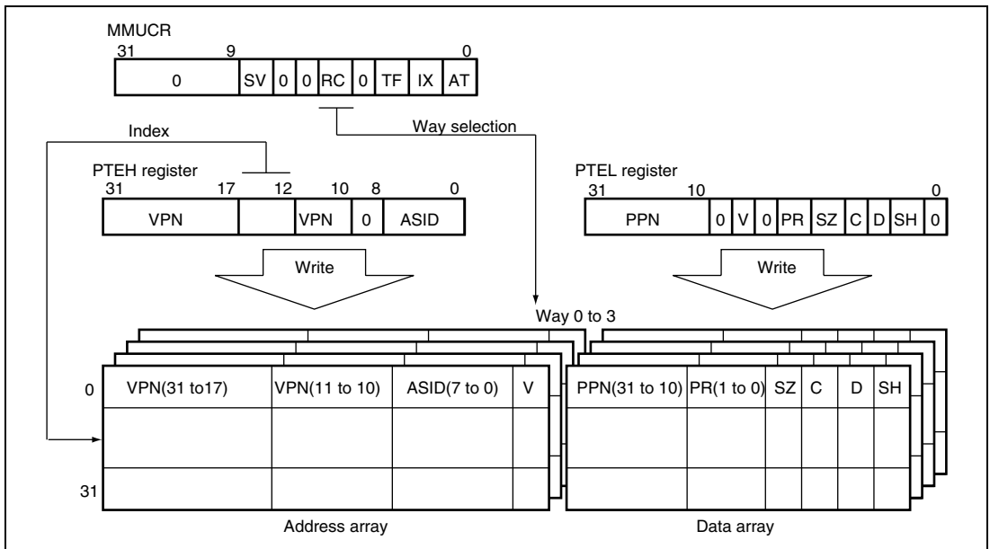
Figure 3.8 Operation of LDTLB Instruction
