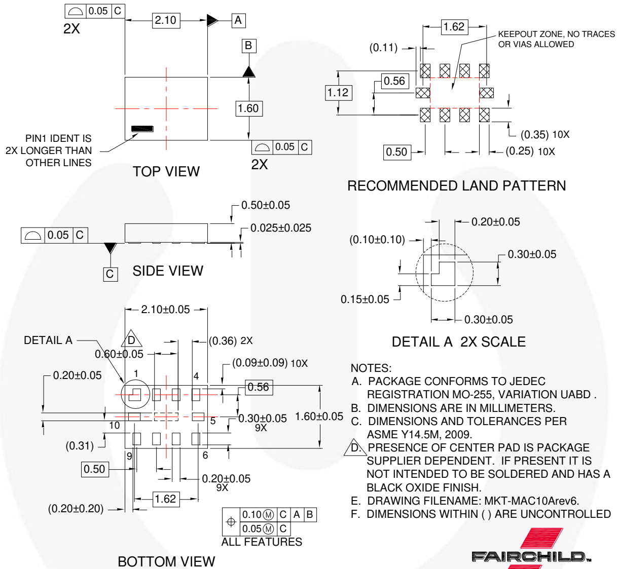
Figure 6. 10-Lead, MicroPak™, JEDEC MO255, 1.6 x 2.1 mm
