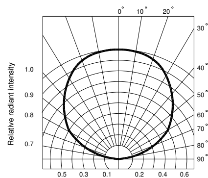
Fig.6 Radiation diagram
