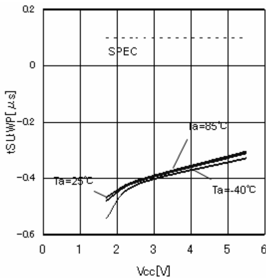
Figure 28. WP setup time t_{\text{SU:WP}}
