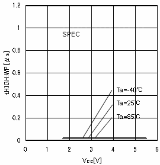
Figure 29. WP valid time t_{\text{HIGH:WP}}
