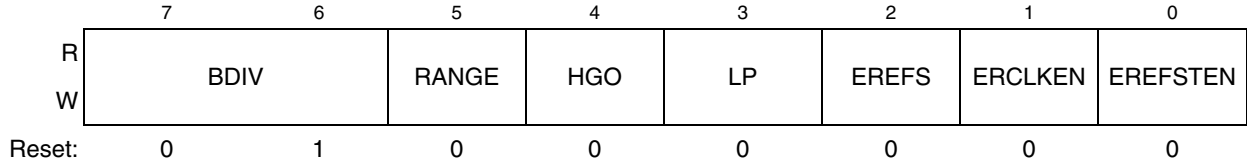
Figure 12-4. MCG Control Register 2 (MCGC2)
