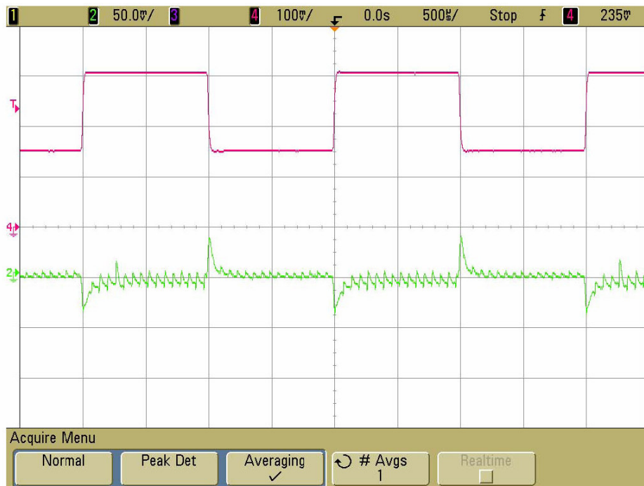
Figure 5. Transient Response Waveform at 4.2Vin and 1.5 - 3.0Aout – 500uS and 50mV / div
