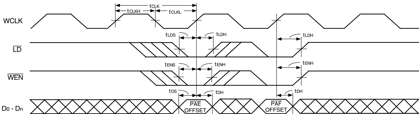
NOTE: 4667 drw21 1. This timing diagram illustrates programming with an input bus width of 36 bits.
