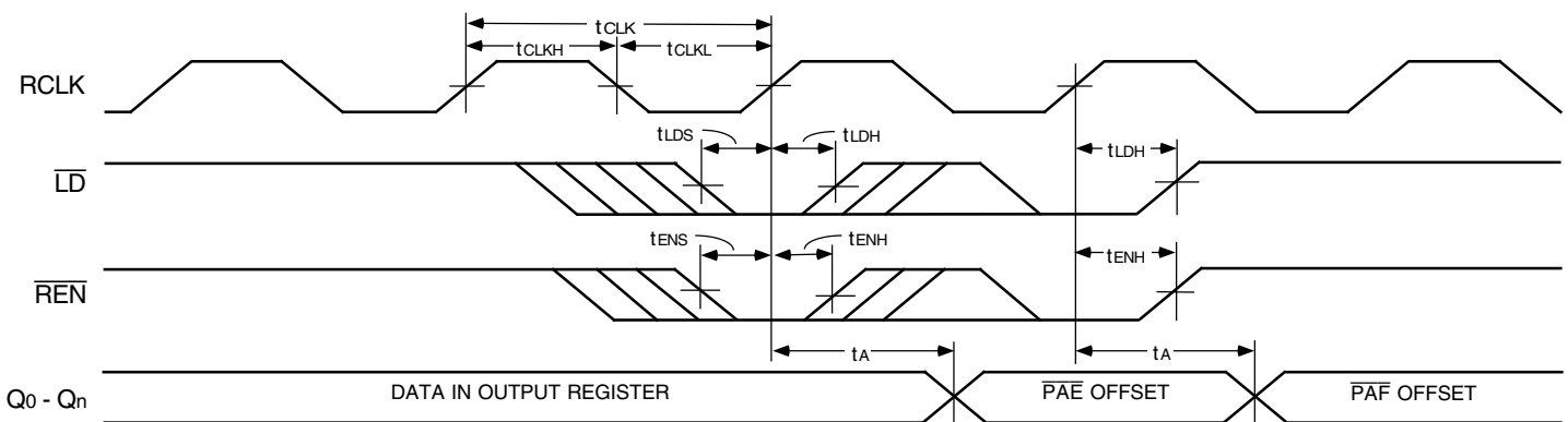
NOTES: 4667 drw22 1. OE = LOW. 2. The timing diagram illustrates reading of offset registers with an output bus width of 36 bits.
