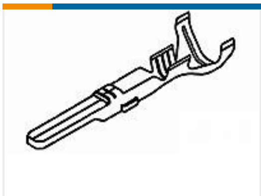
TE Part #881590-1 ECONOSEAL TAB .070
