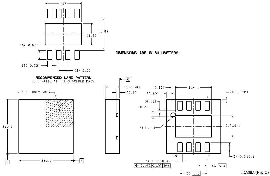
LLP-8, 3mm x 3mm Body Order Number DS90LV012ATLD, DS90LT012ATLD NS Package Number LDA08A
