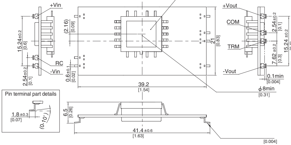
1.SMD(type B)
