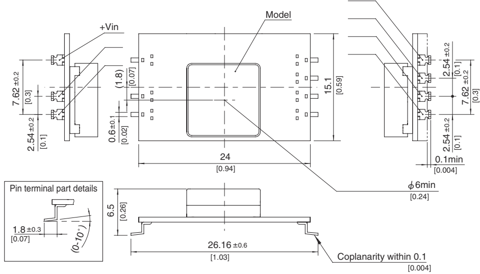
1.SMD(type B)
