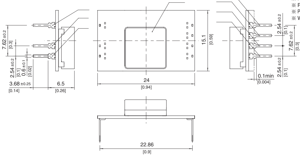
2.DIP(type C)
