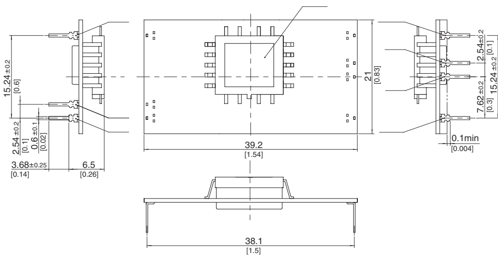
2.DIP(type C)
