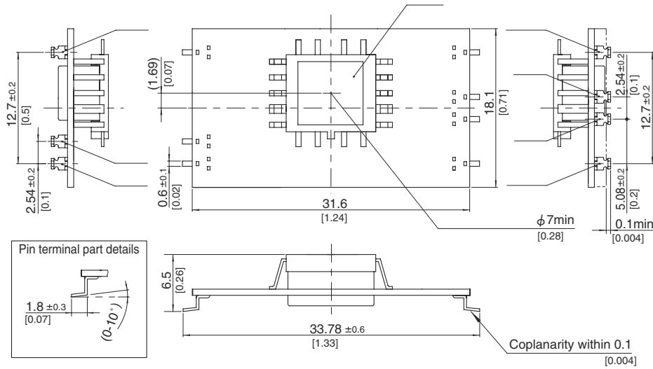
1.SMD(type B)
