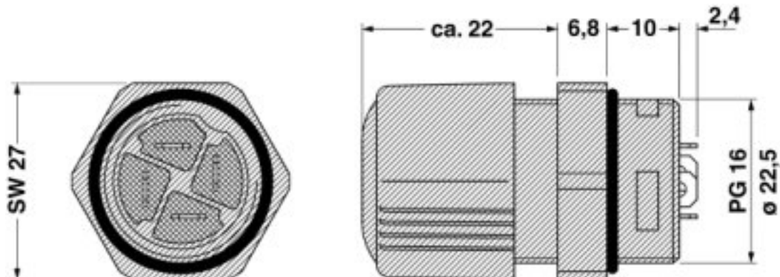
Dimensioned drawing
